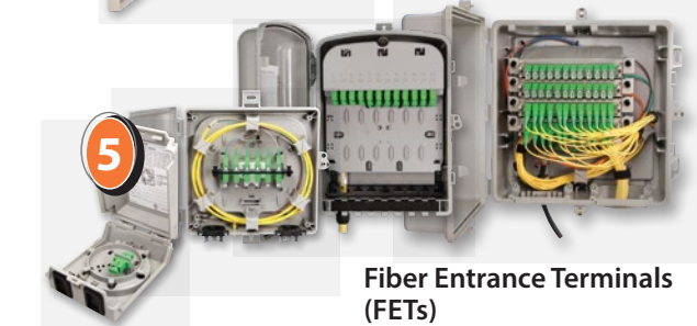
4 Fiber Distribution Hubs (FDH)
