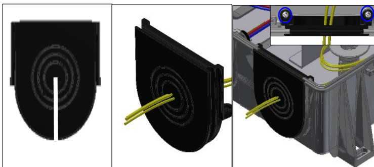
15. CUT THE GROMMET FROM ROUND SIDE TO THE CENTER AS SHOWN, INSTALL THE PORT CAP INTO THE BASE OPENING WITH 2 SCREWS.
