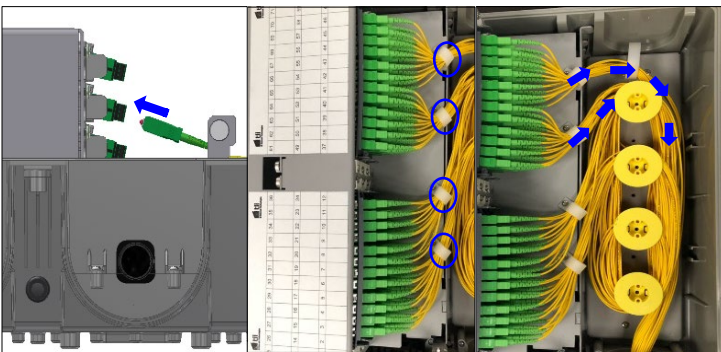
13. PLUG THE CONECTORS AND THEN ROUTE FIBERS
