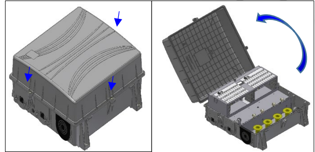
2. LOOSEN SCREWS AND OPEN THE COVER
