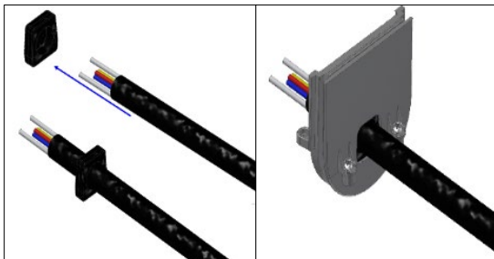
5. MAKE A CUT ON THE GROMMET, INSTALL OVER CABLE AND ASSEMBLE PORT CAP.
