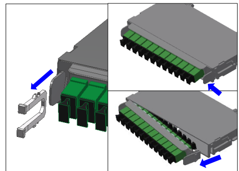
14. IF REAR ACCESS TO BULKHEAD IS NEEDED, REMOVE CLIP, PUSH EITHER TAB ON THE BULKHEAD AND REMOVE
