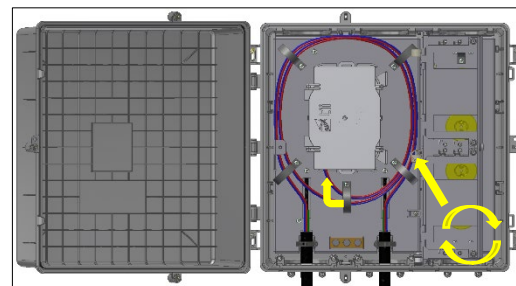
8. ROUTE FIBER INTO THE CLIPS USING PROTECTIVE SLEEVES AND THEN FEED SPLICE TRAY
