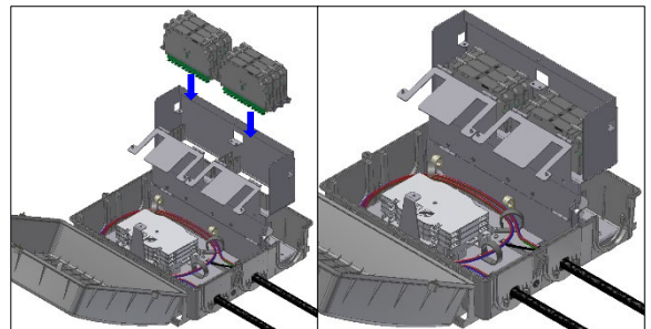
10. INSERT THE CASSETTES
