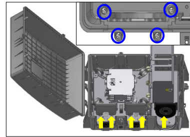
4. REMOVE SCREWS AND PORT CAPS
