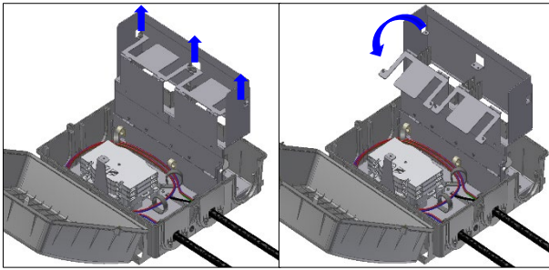
9. LOOSEN THE THUMB SCREWS AND OPEN THE LOCKING BRACKET
