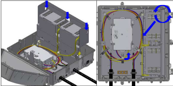
11. CLOSE THE LOCKING BRACKET WITH THE SCREWS AND ROUTE THE FIBER IN THE CLIPS AND THEN INTO THE SPLICE TRAY
