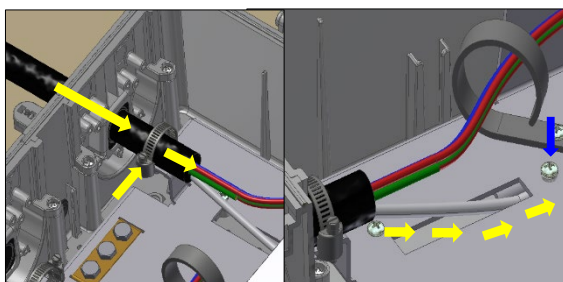
CLAMP CABLE JACKET
