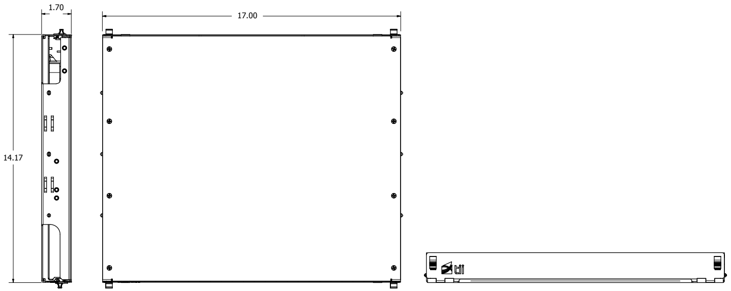
Dimensions are in Inches
